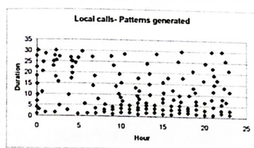
Fig. 2. Patterns generated after the training corresponding to local calls
