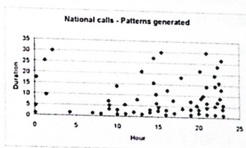
Fig. 3. Patterns generated after the training corresponding to national calls
