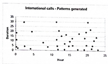
Fig. 4. Patterns after the training corresponding to international calls
